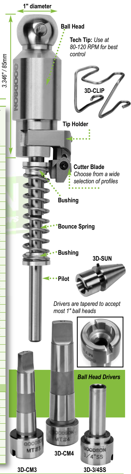
Ball Heads
